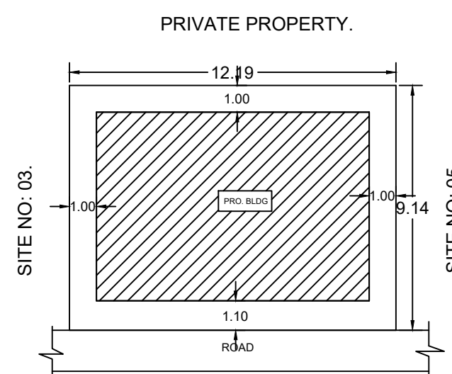
SITE PLAN
