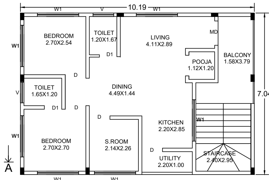
TYP: GROUND & FIRST FLOOR PLAN
